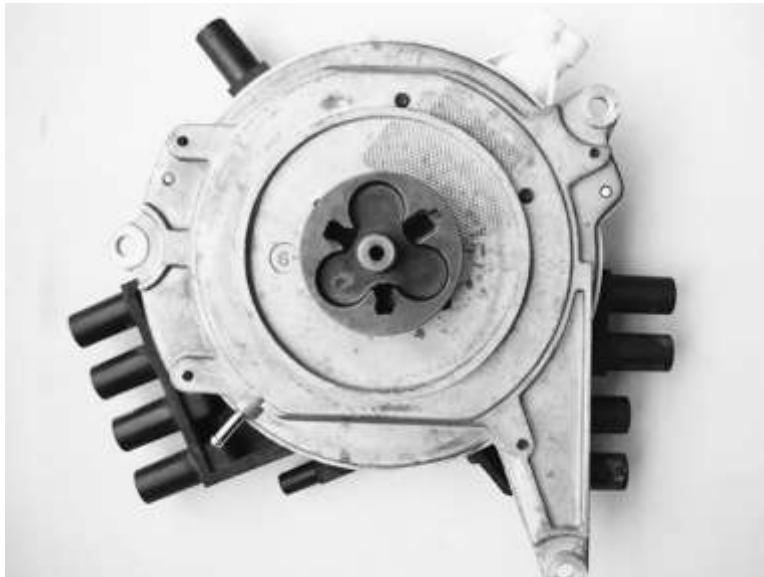
The revised version has a larger cam drive mechanism and an additional metal vent on the case of the distributor.
