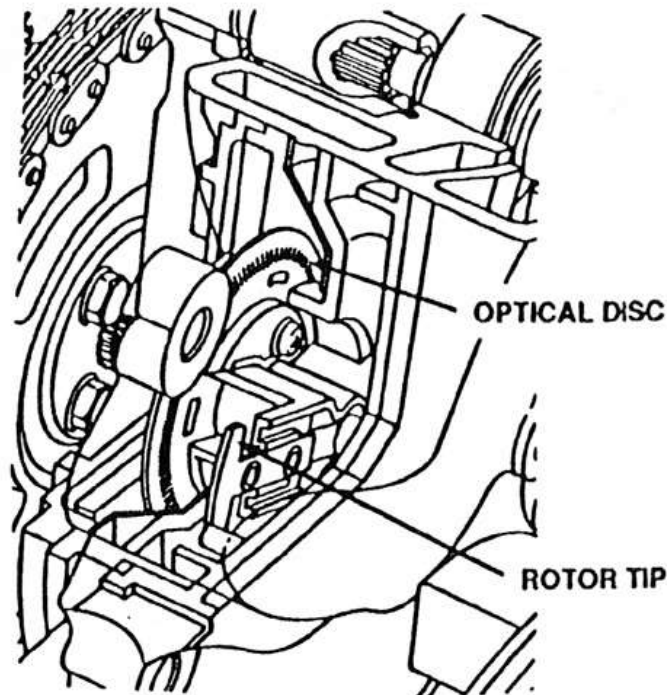
FIGURE 37 OPTI-SPARK CONFIGURATION
