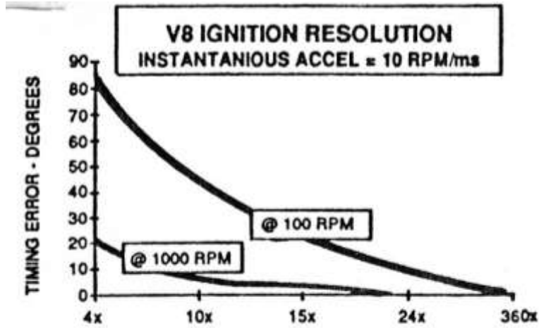
FIGURE 41 ECM REFERENCES/REVOLUTION
